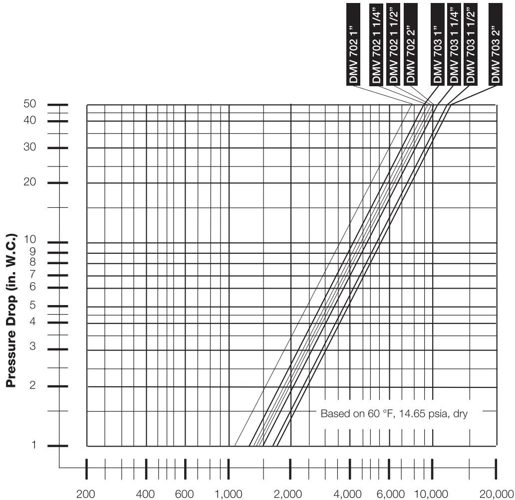
Flow (CFH) of natural gas s.g. 0.65 at 60 °F 20 in W.C. Inlet
